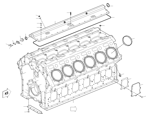
CRANKCASE UPC.06A01 2075
